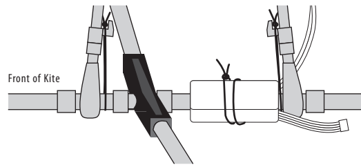
Battery Placement for Tail Heavy Flying
